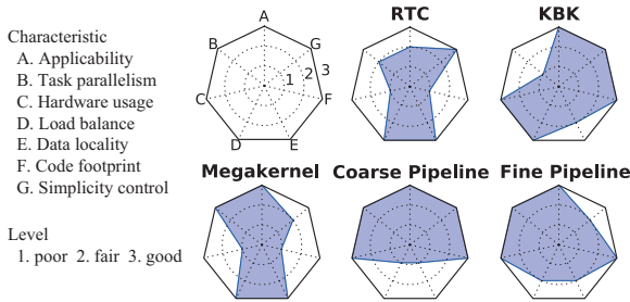
Figure 6: Characteristics of each pipeline model.
