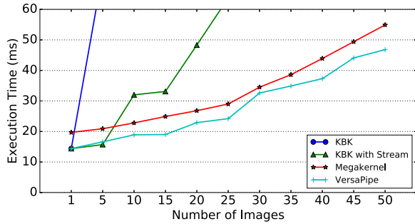
Figure 13: Performance results of Image Pyramid.
