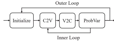
Figure 17: The pipeline structure of LDPC.
